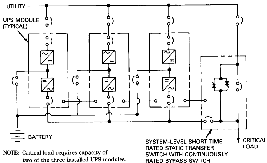
Figure 41—Parallel Redundant UPS System
