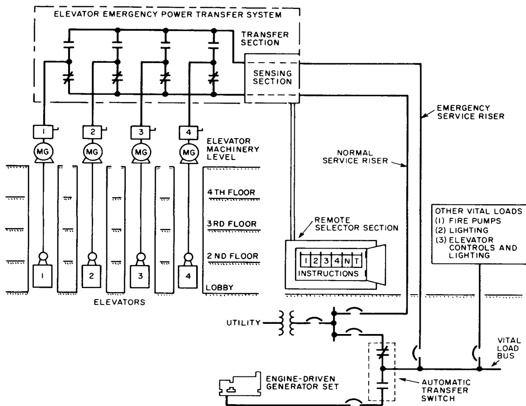
Figure 149—Typical Standby Power Transfer System
